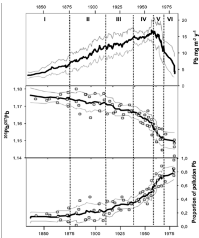
Lead accumulation and isotopic composition in cores collected in Chao de Lamoso (Xistral Mountains, NW Spain), showing the evolution of metal atmospheric pollution in the last few centuries. Modified from Martínez Cortizas et al., (2012) 29
